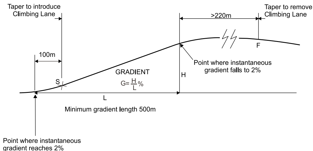
Figure 5/3: Layout of Climbing Lane - Extended (Terminating beyond 220m from the 2% point on the Crest Curve)
